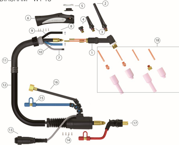
DIAGRAM WT 18
