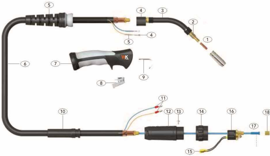
DIAGRAMA WCM 150
